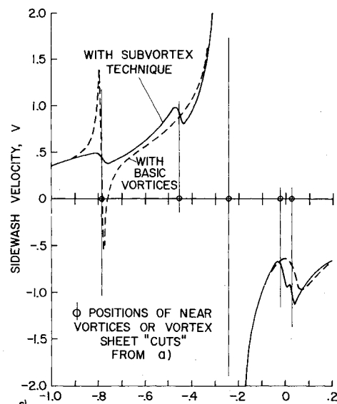
Fig. 6 Simple application of the subvortex technique to the vortex sheet rollup calculation in two dimensions. a) Calculated vortex positions after 20 time steps ( t=1.5 ). b) Calculated upwash distribution. c) Calculated sidewash distribution.
