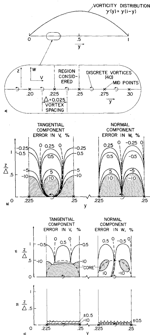
Fig. 3 Velocity error calculations. a) Location of region considered. b) Error contours for the basic discretization. c) Error contours for two near-field models: 1) core model (Rankine vortex); core diameter = \Delta . 2) subvortex technique; near-field radius = 5\Delta . NSC_{max} = 10 .
