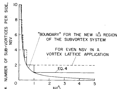
Fig. 4 Subvortex technique. a) Arrangement of the subvortices for NSV=4 . b) Number of subvortices as a function of height above the segment.
