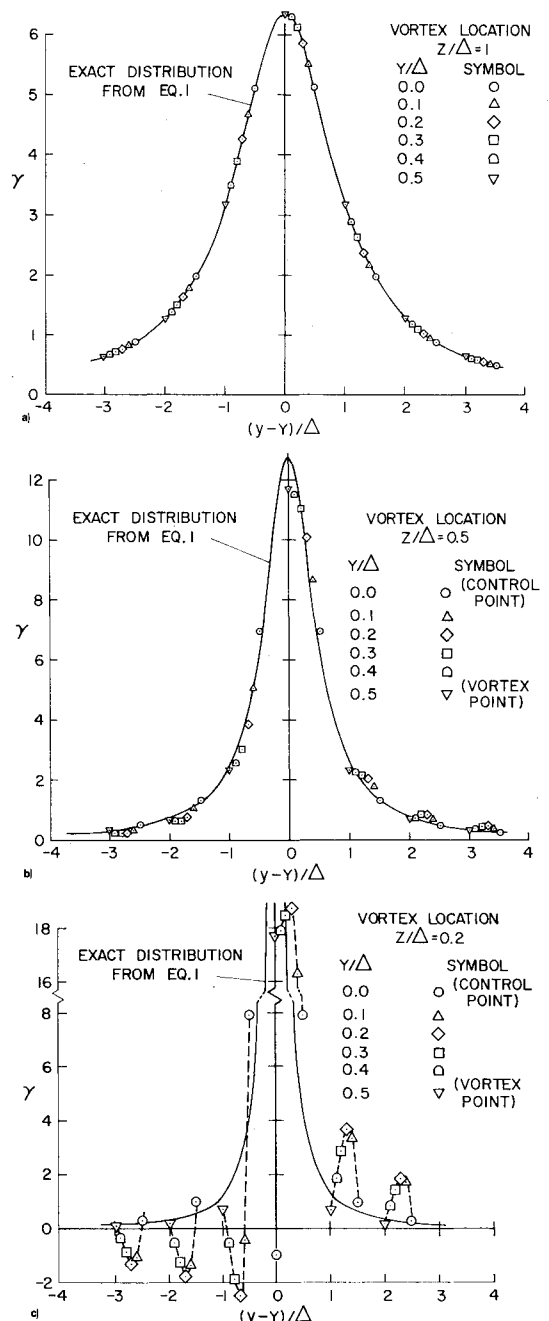
Fig. 2 Vorticity induced on a plane surface by a vortex - effect of vortex location on discretized solution. a) Vortex height Z=\Delta . b) Vortex height Z=0.5\Delta . c) Vortex height Z=0.2\Delta .
