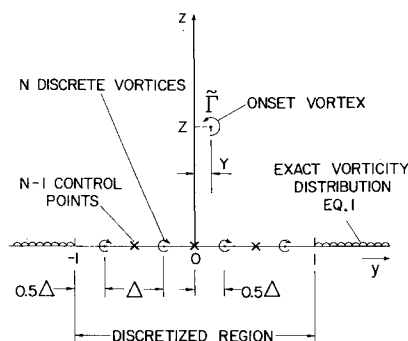
Fig. 1 Vorticity induced on a plane surface by a vortex - discretized model.
