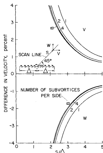
Fig. 5 Subvortex technique. Difference between velocities from subvortices and from the basic vortex.
